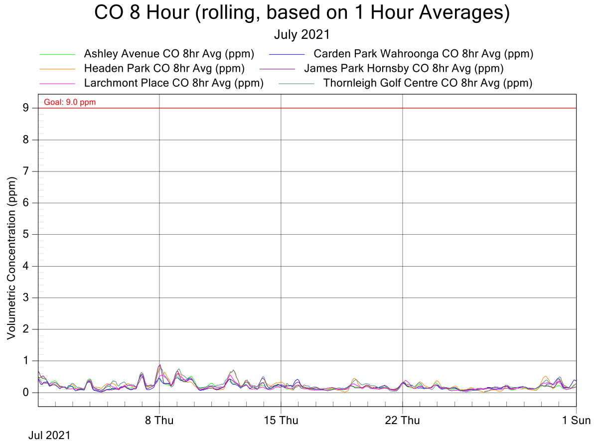
Figure 2: NorthConnex Project Air Monitoring Stations - CO 8 Hour Rolling Averages for July 2021
