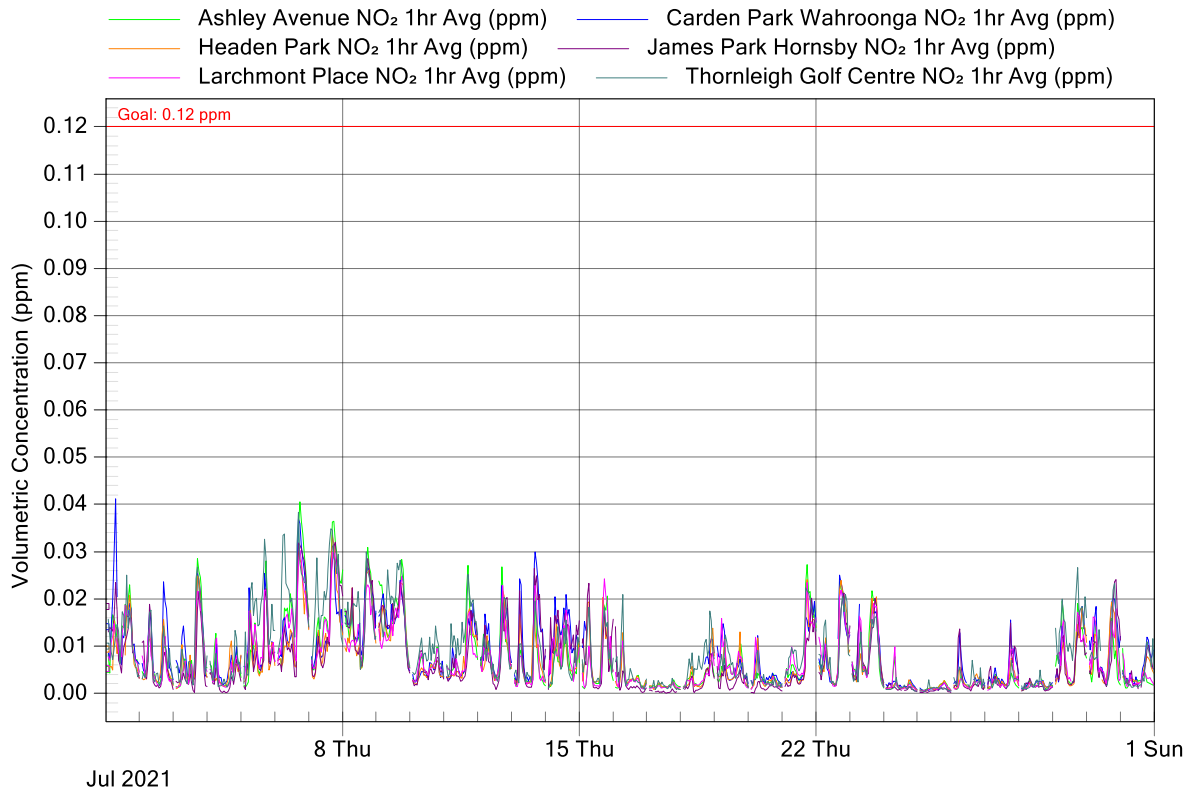
Figure 3: NorthConnex Project Air Monitoring Stations - NO 2 1 Hour Averages for July 2021
